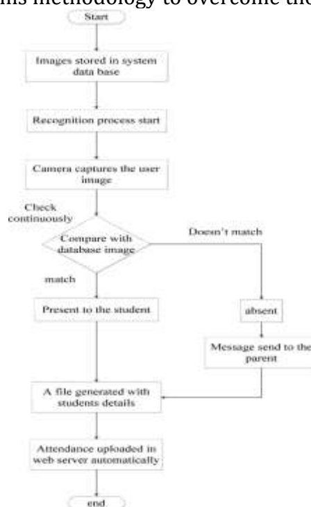
Figure 1: Diagram of Proposed System
