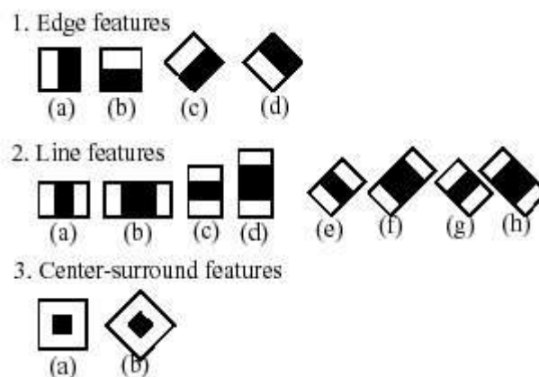
Figure 2: Sorts of Haar Features
