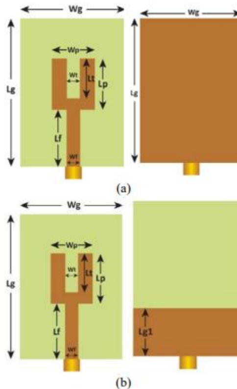
Fig 1. Antenna's Layout (A) TFS (B) PG-TFS
